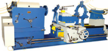
LATHE MACHINE PLANNER TYPE CENTRE 16" / 18" / 20" / 22" / 24" / 26" / 28" 406MM / 457MM / 508MM / 559MM / 610MM / 660MM / 711MM
